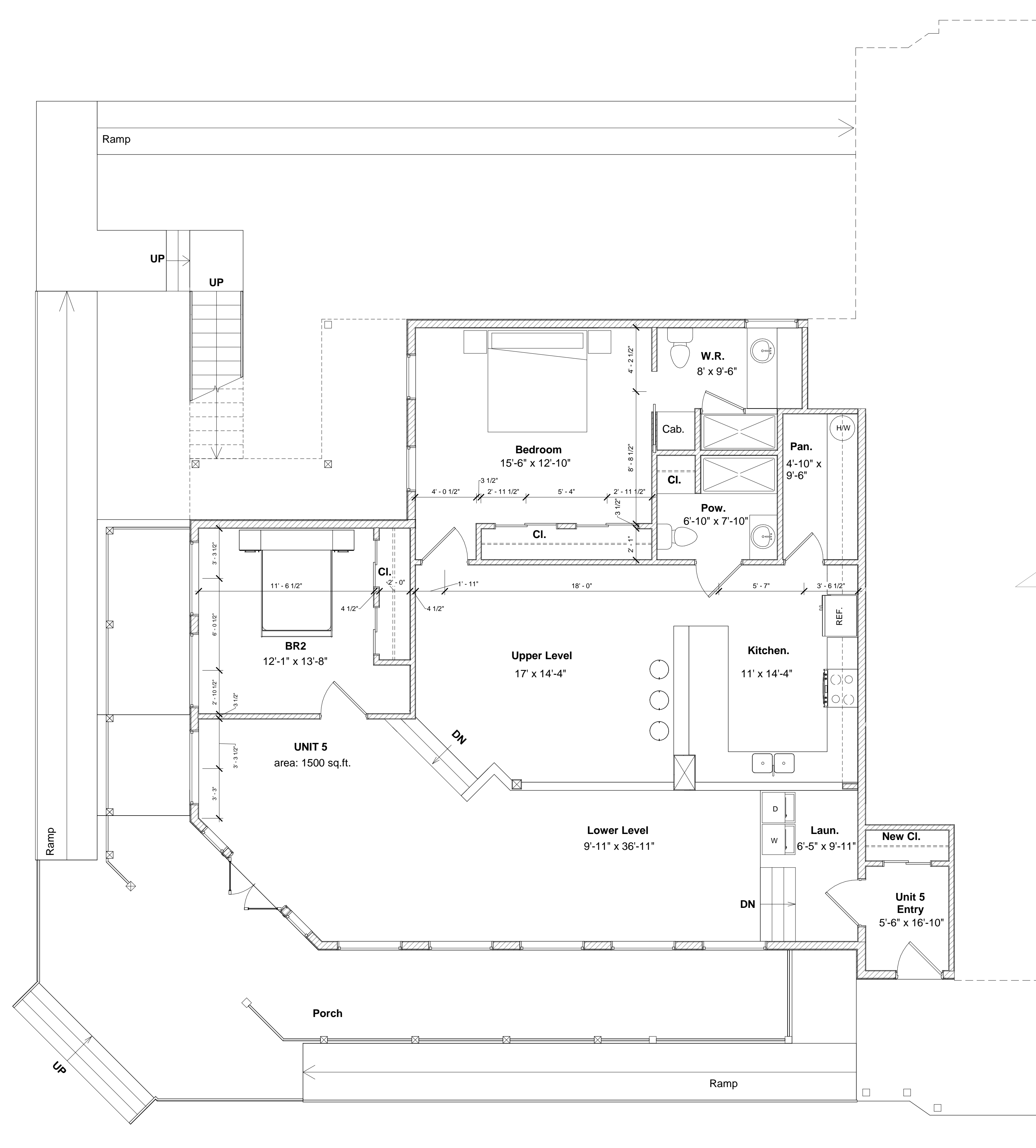
① Unit 5 1/4" = 1'-0"
