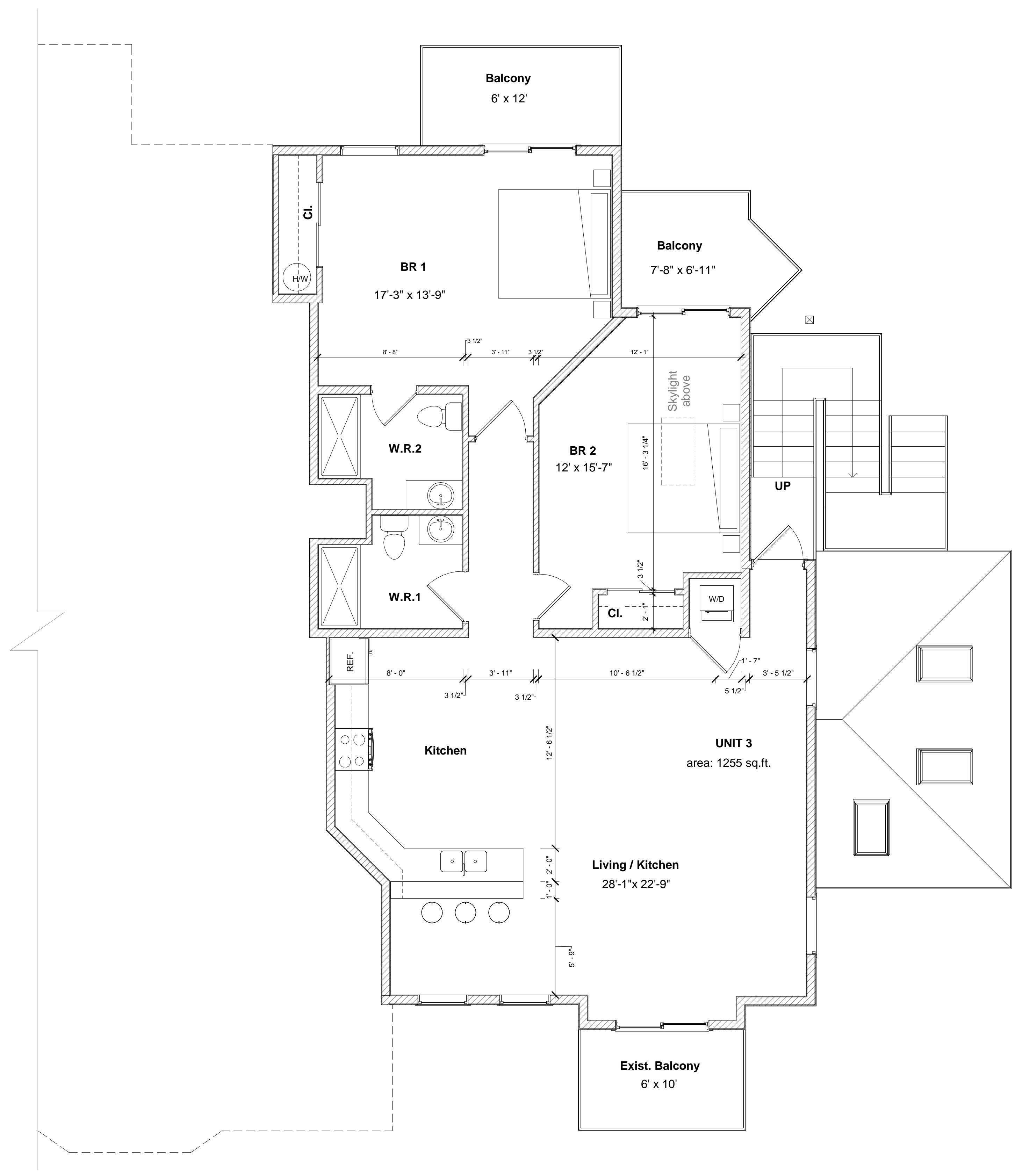
① Unit 3 1/4" = 1'-0"
