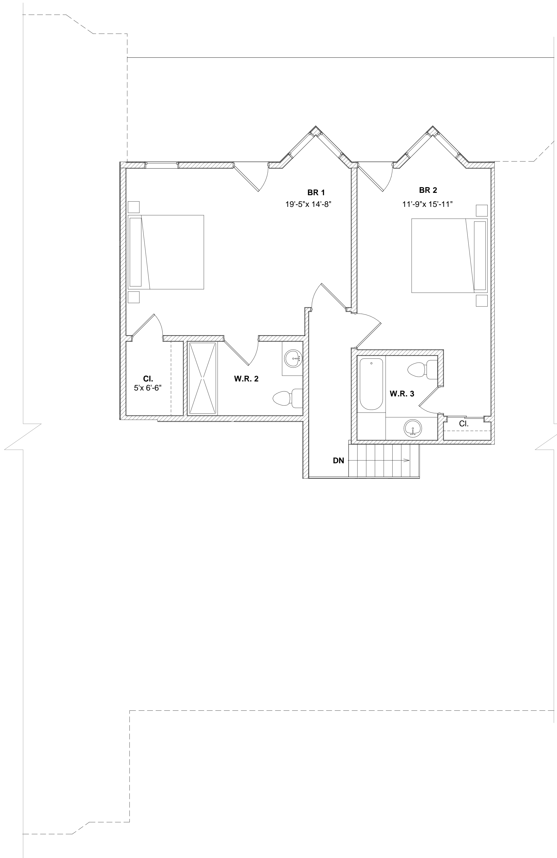
② Unit 2 Upper Level 1/4" = 1'-0"
